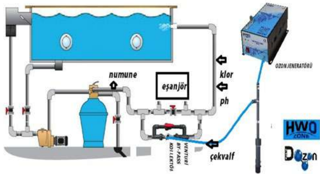
Evsel Havuzlar İçin Venturi By-Pass Montaj Şema Venturi For Domestic Pools By-Pass Installation Diagram
